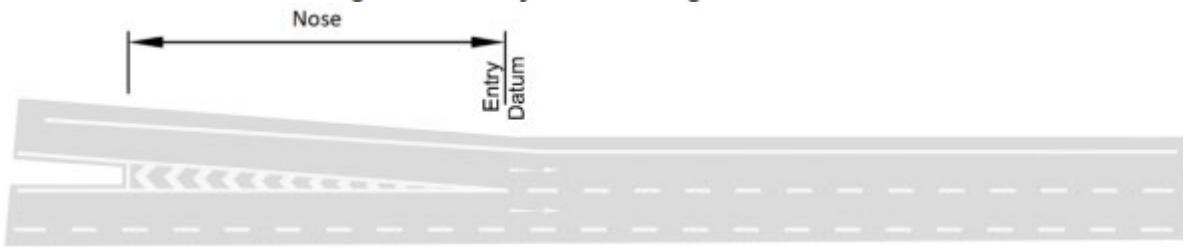
Figure 3.14e Layout D - lane gain
