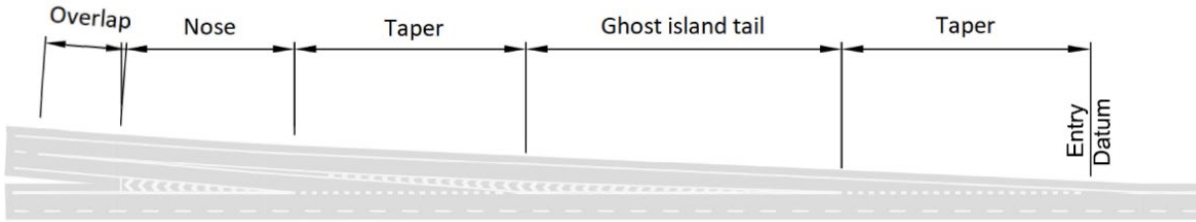
Figure 3.14e Layout D - lane gain
