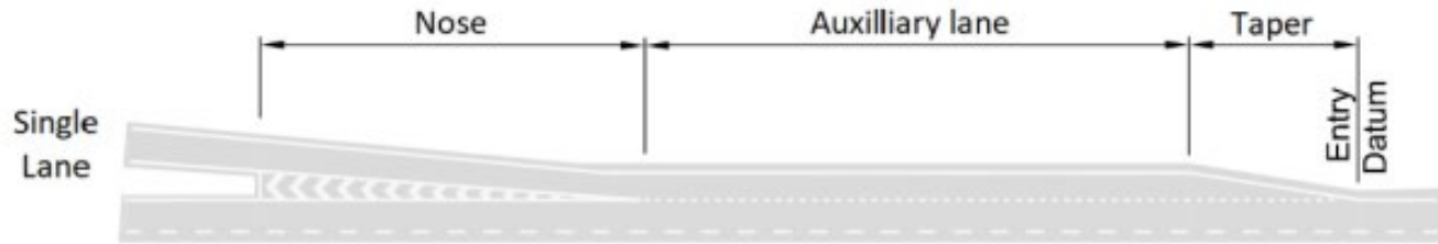
Figure 3.14d Layout C - ghost island merge
