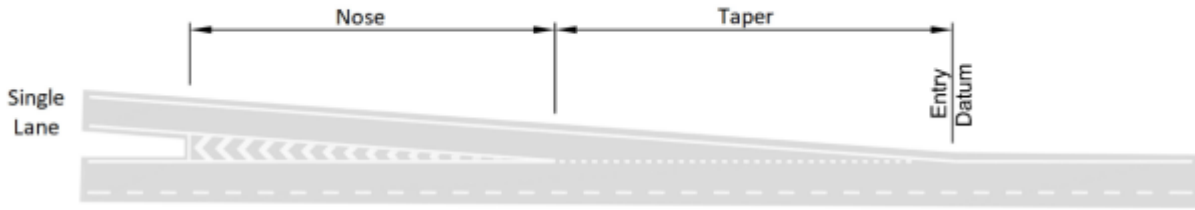
Figure 3.14c Layout B - parallel merge
